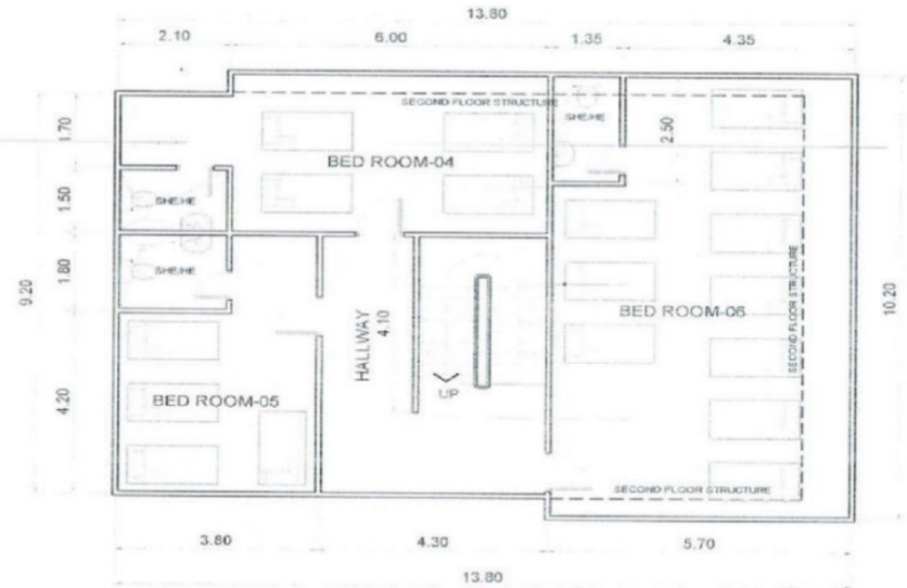
THIRD FLOOR PLAN SCALE 1 : 100 M
